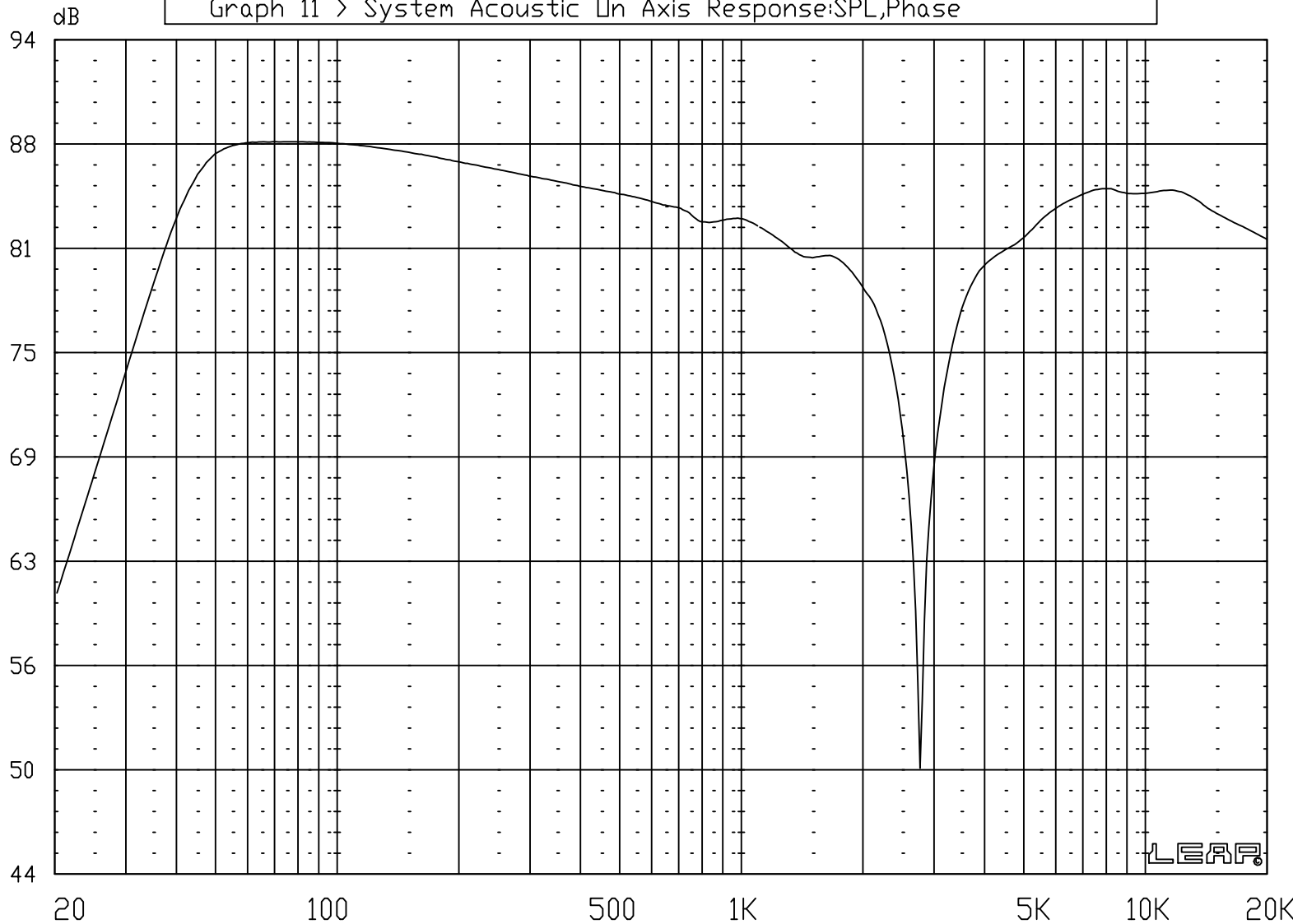
Graph 11 > System Acoustic On Axis Response:SPL,Phase
