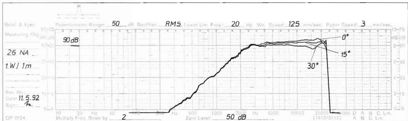
Frequency Response
