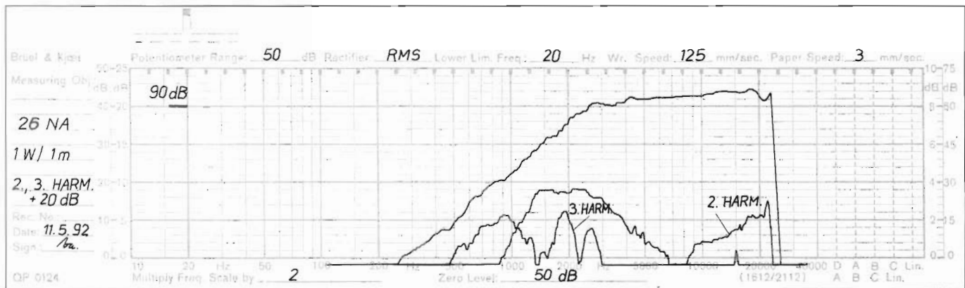
Frequency Response/Distortion
