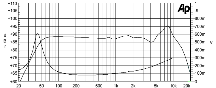
AUDIO PRECISION : W14RC25-08
