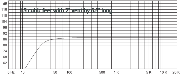
Custom Amplitude Response (dB-SPL/Hz at 1 m) with 1 watts BassBox 6 Pro
