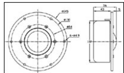
DMA-A Mechanical Drawing (Magnify)
