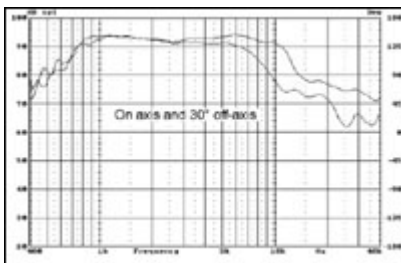
DMA-A Frequency Response (Magnify)
