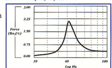
Bass Shaker Frequency Response
